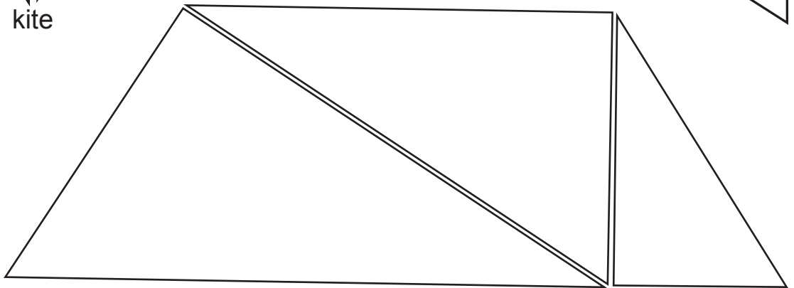
trapezoid
