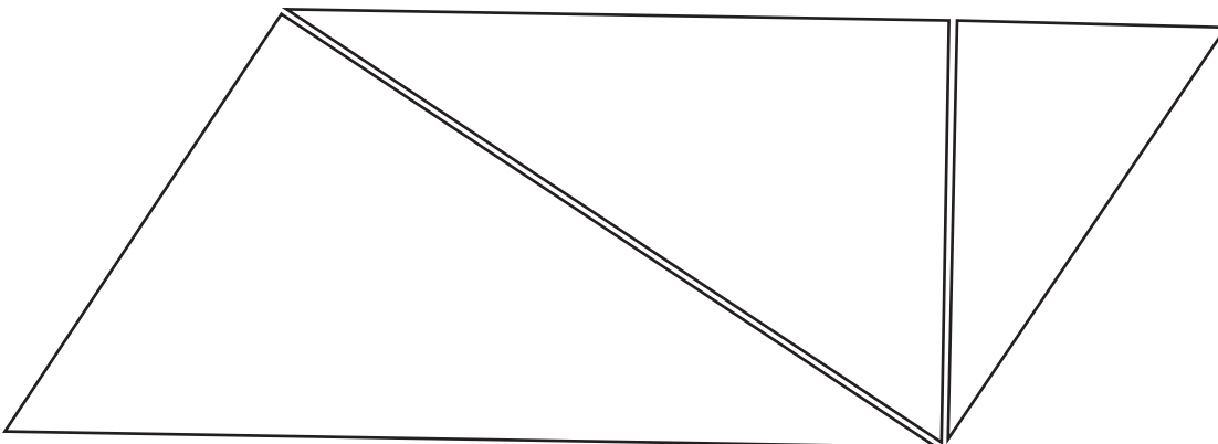
parallelogram
