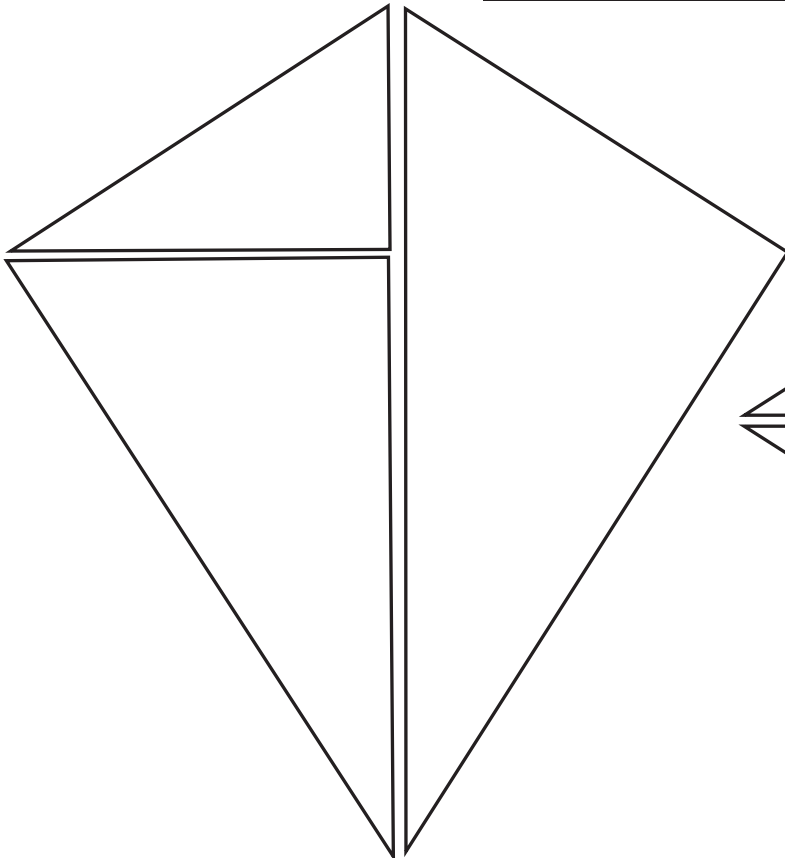
kite
