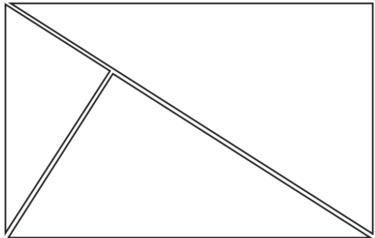
rectangle
